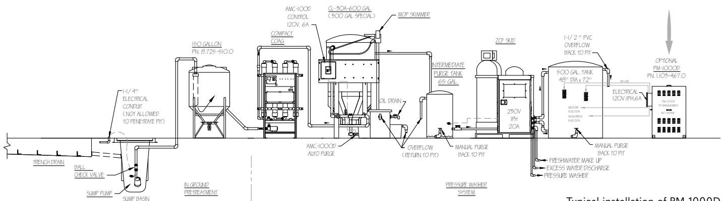
Typical installation of PM-1000D
